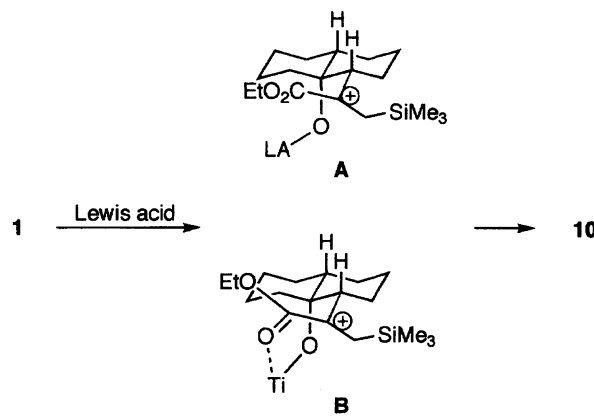
Scheme 6.
